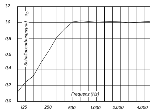
Screen50 Wandabsorber
